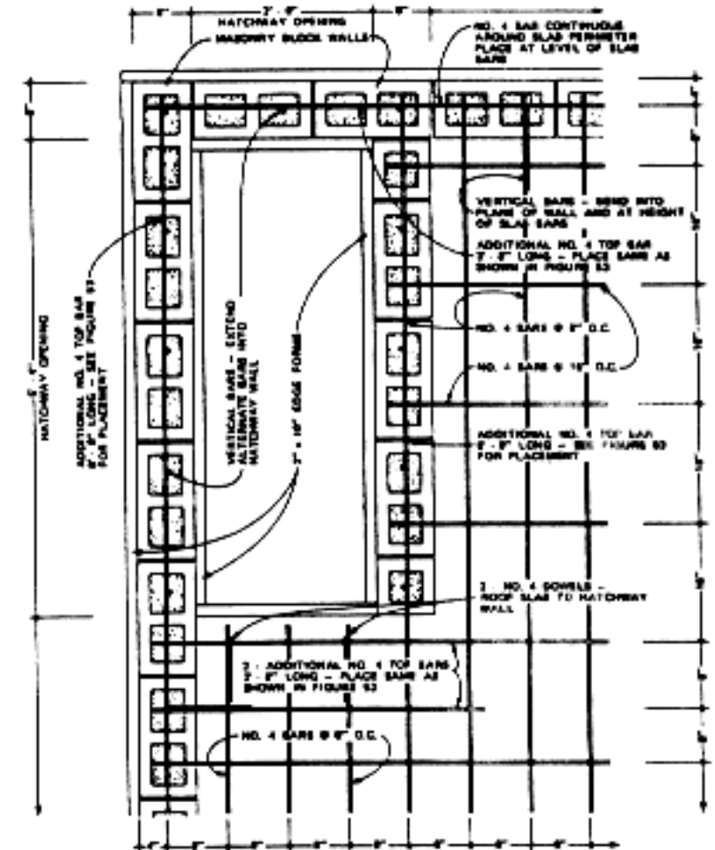
Figure 56. Roof slab edge reinforcement around hatchway
