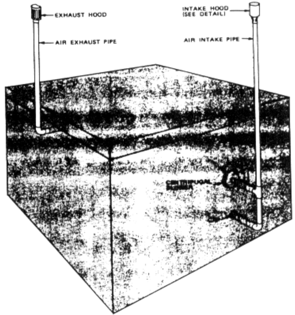
Fabrication 15. Piping diagram of ventilation system
