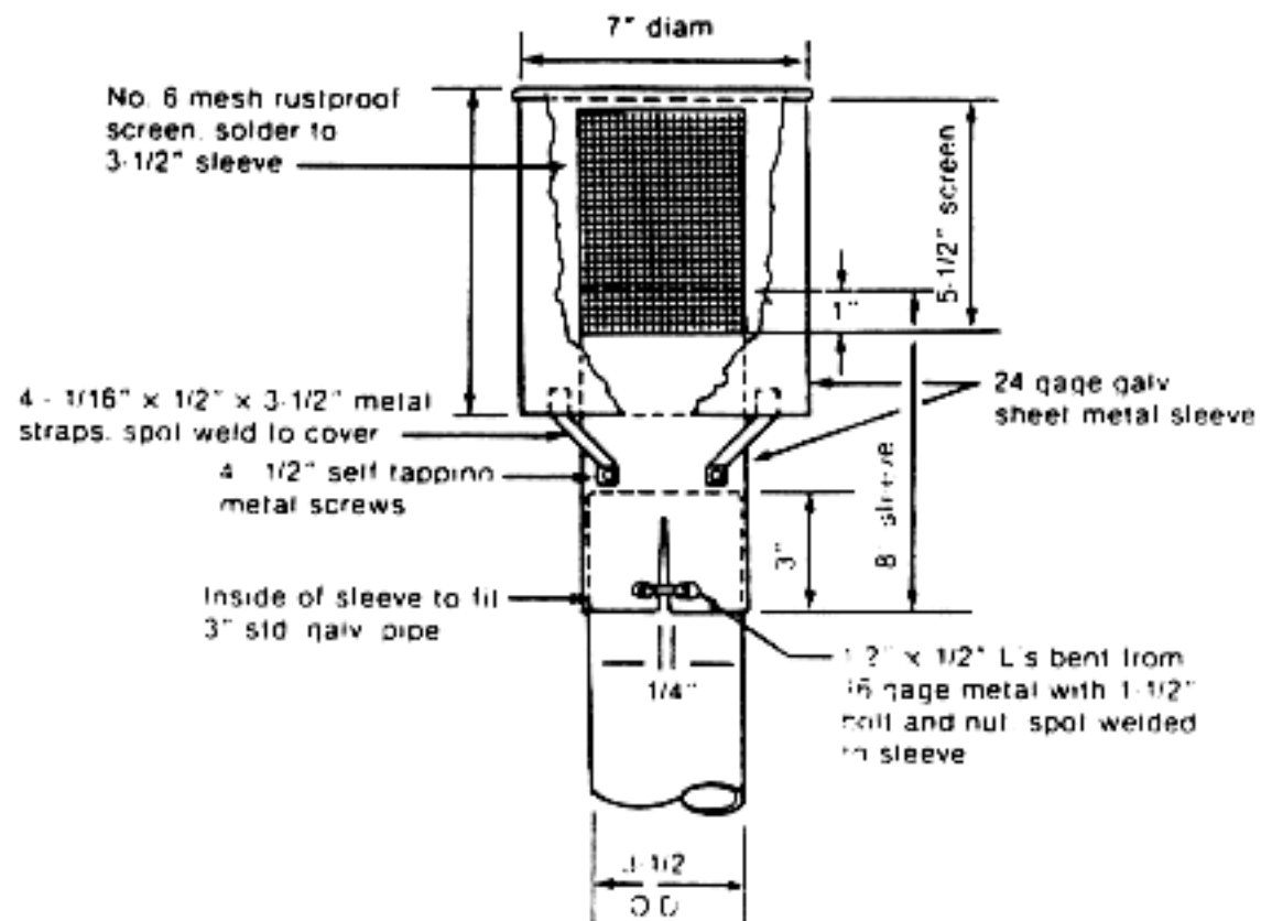
Air Intake Hood Details
