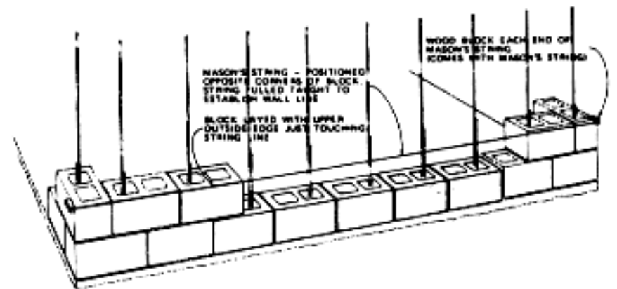
Figure 47. Infill block units in wall between corners
