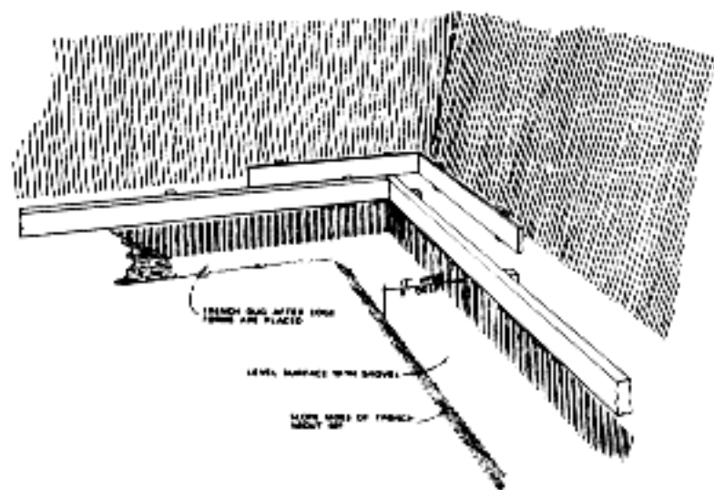
Figure 26. Trench for the thickened slab edges
