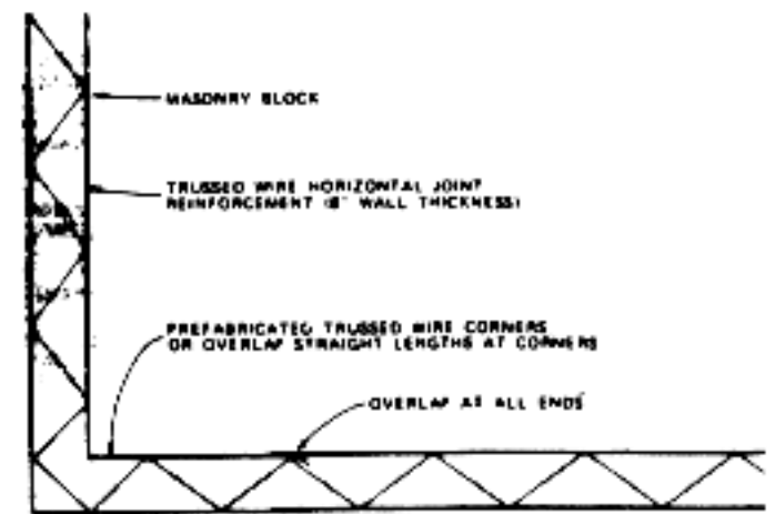
Figure 39. Placement of reinforcement in masonry wall
