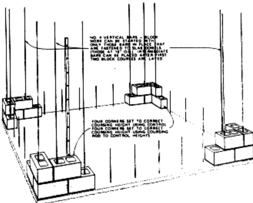
Figure 46. Corners of the shelter set for first two block courses
