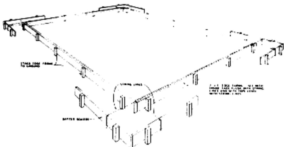
Figure 25. Placement of edge forms for floor slab
