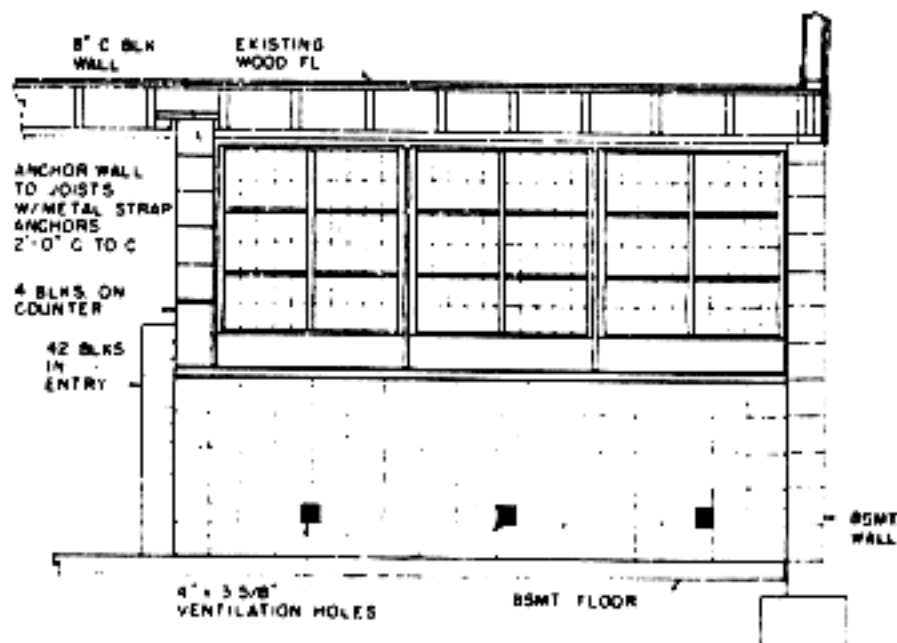
Section B
