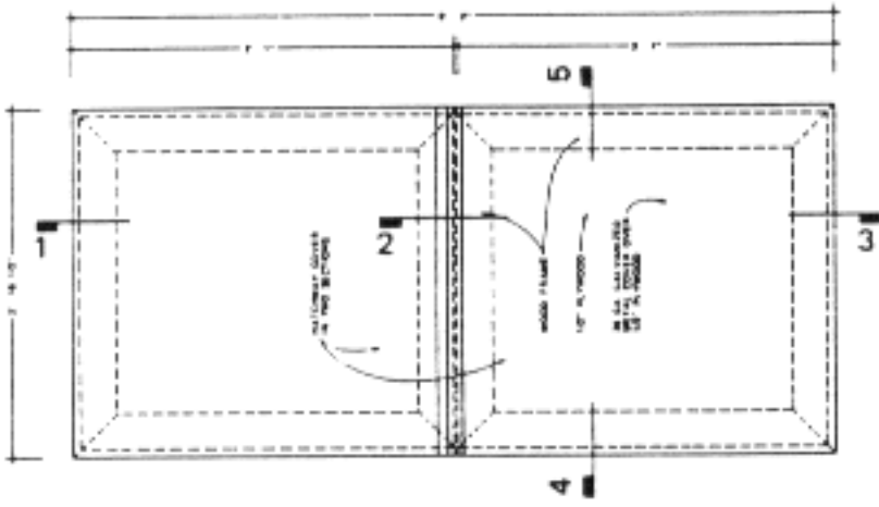
Figure 12. Construction dimensions of hatchway cover
