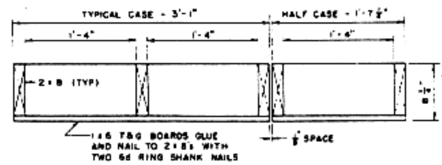
Detail Sections
