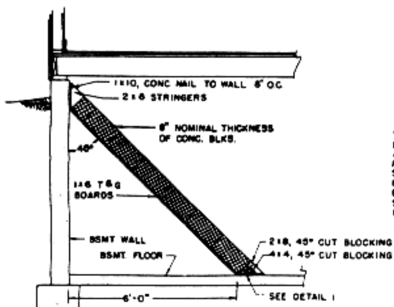
Section A
