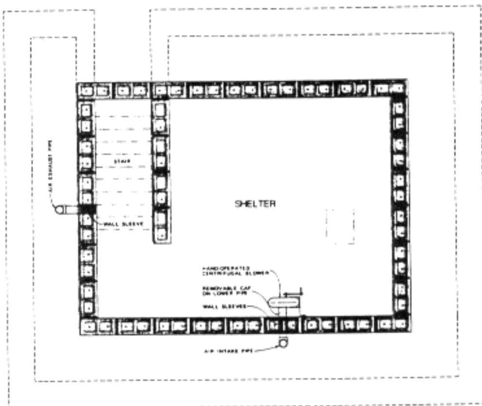
Figure 14. Plan diagram of ventilation system for shelter
