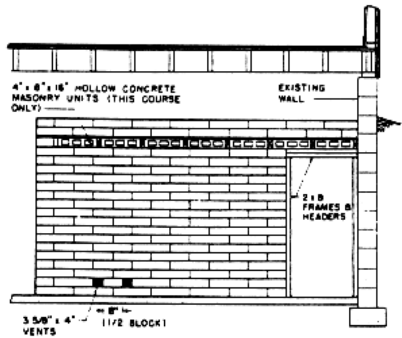
Section B
