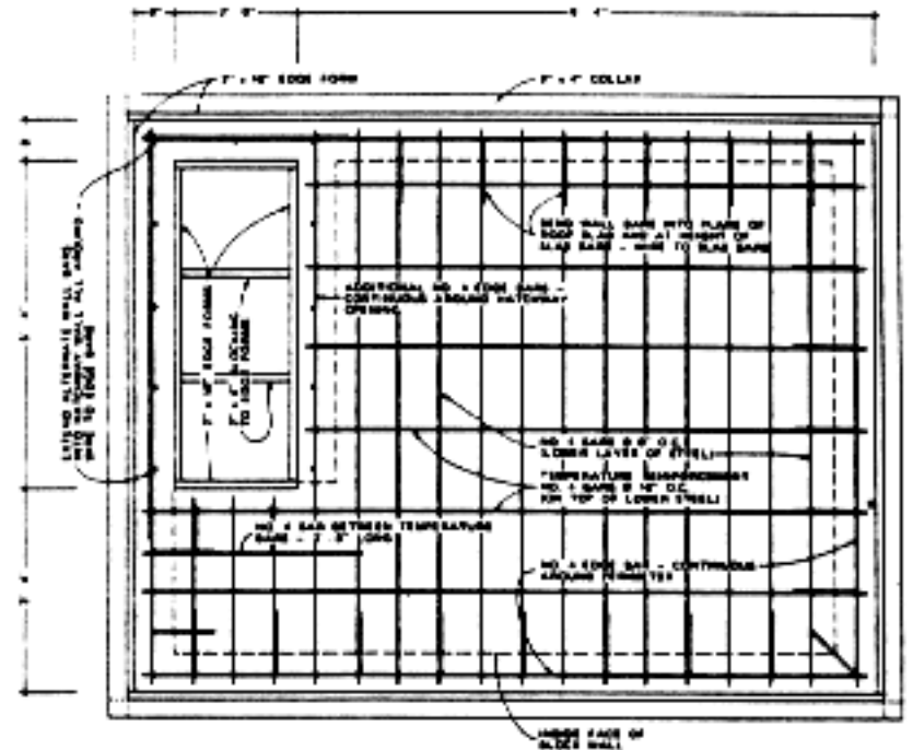
Figure 55. Plan view of roof slab reinforcement steel
