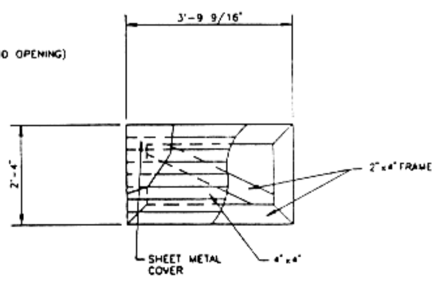
Access Hatch Cover Detail E
