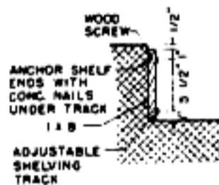
Plan detail of shelf support
