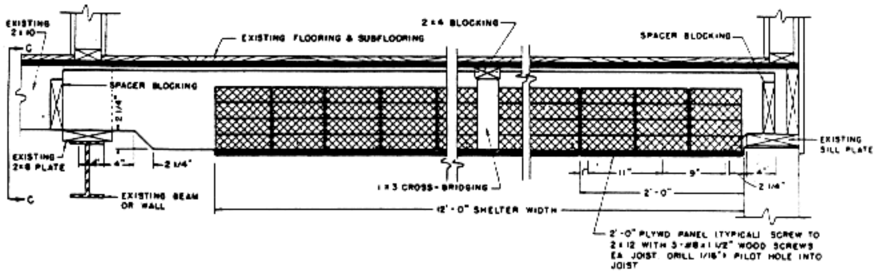
Section B
