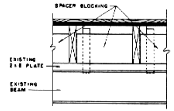
Section C
