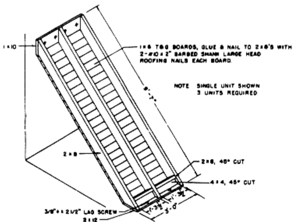
Isometric of Lean-To Unit
