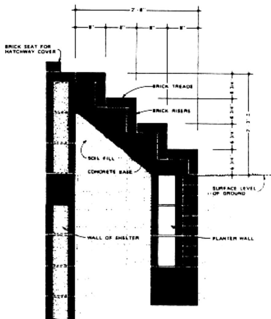
Figure 69. Cross section through brick steps
