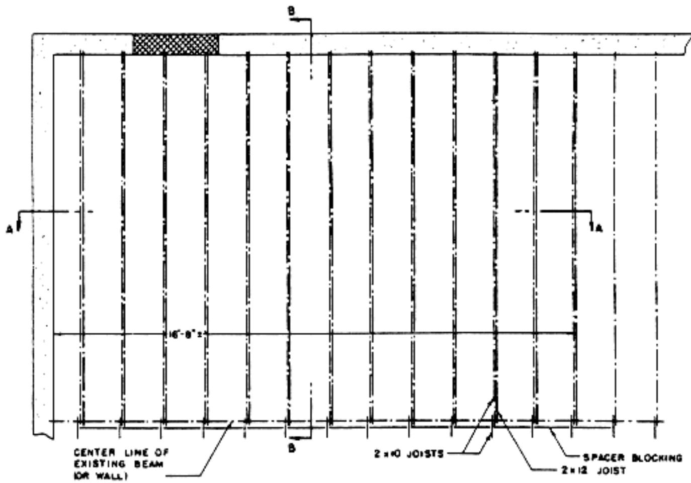
Plan for 12 X 16 Shelter
