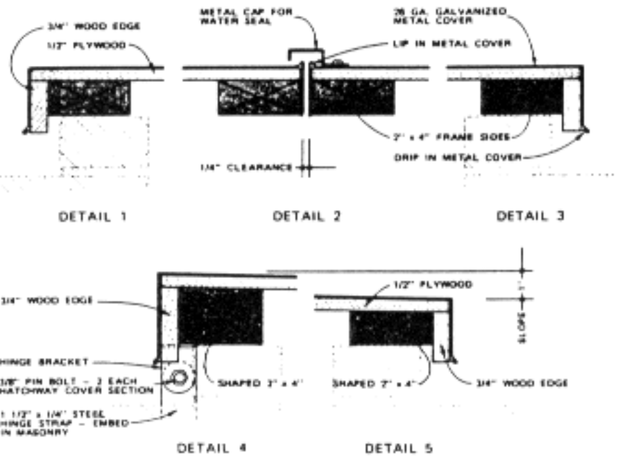
Figure 13. Construction details of hatchway cover
