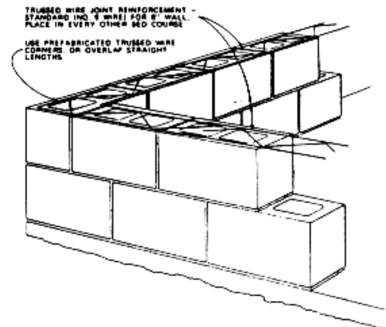
Figure 40. Placement of horizontal joint reinforcement
