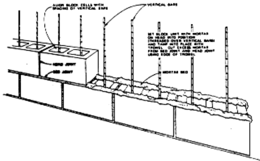
Figure 44. Placement of mortar for bed course of masonry walls
