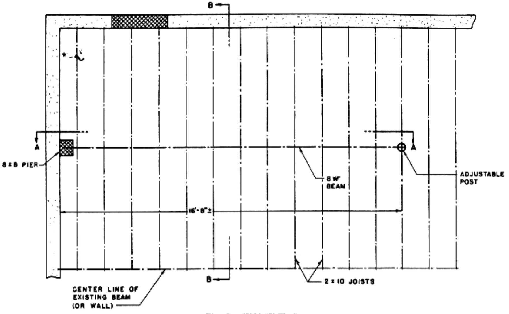
Plan for 12 X 16 Shelter
