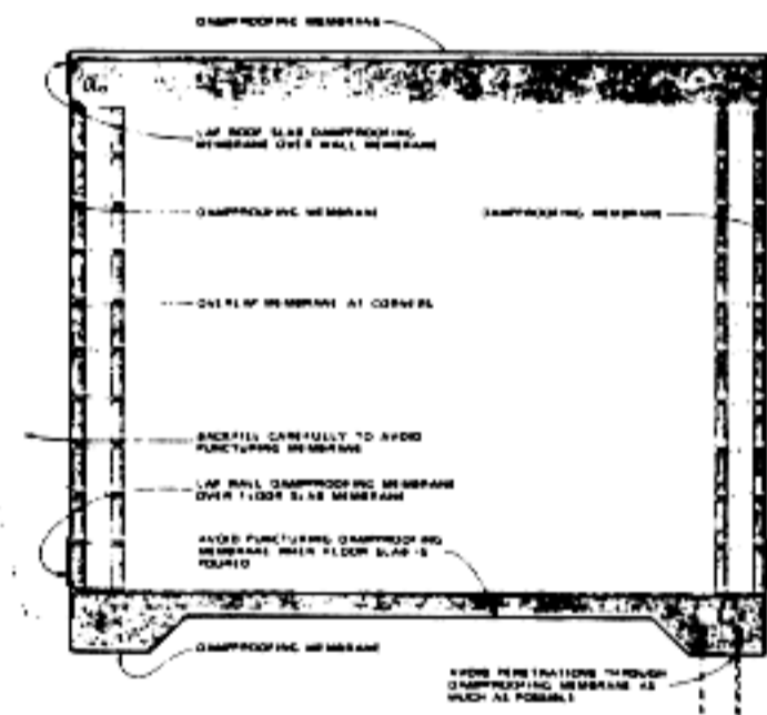
Figure 59. Schematic concept of dampproofing for the structure
