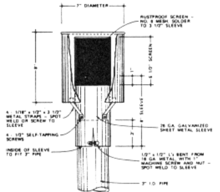
Figure 16. Fabrication of air intake system
