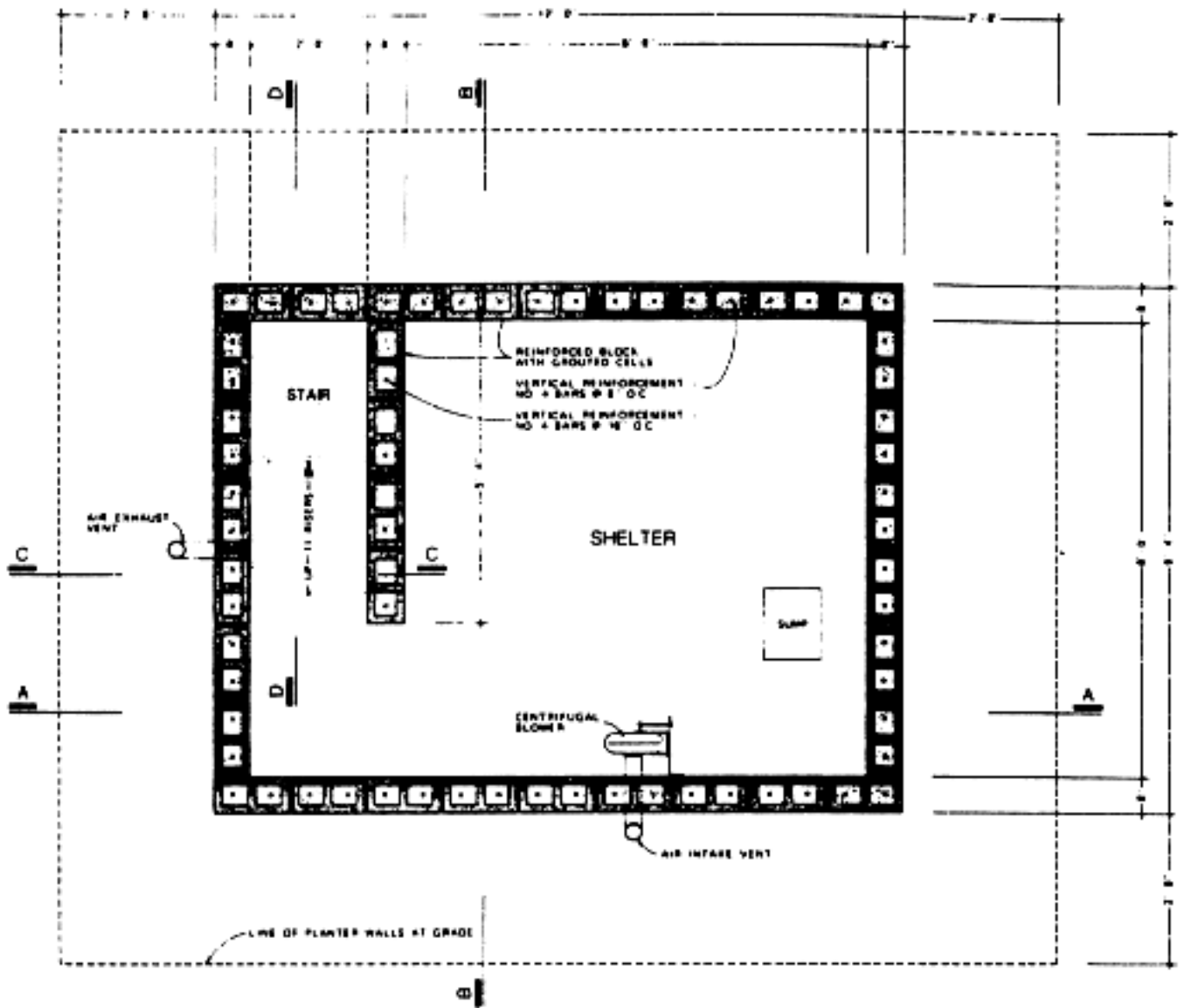
Figure 5. Dimensioned floor plan of the shelter
