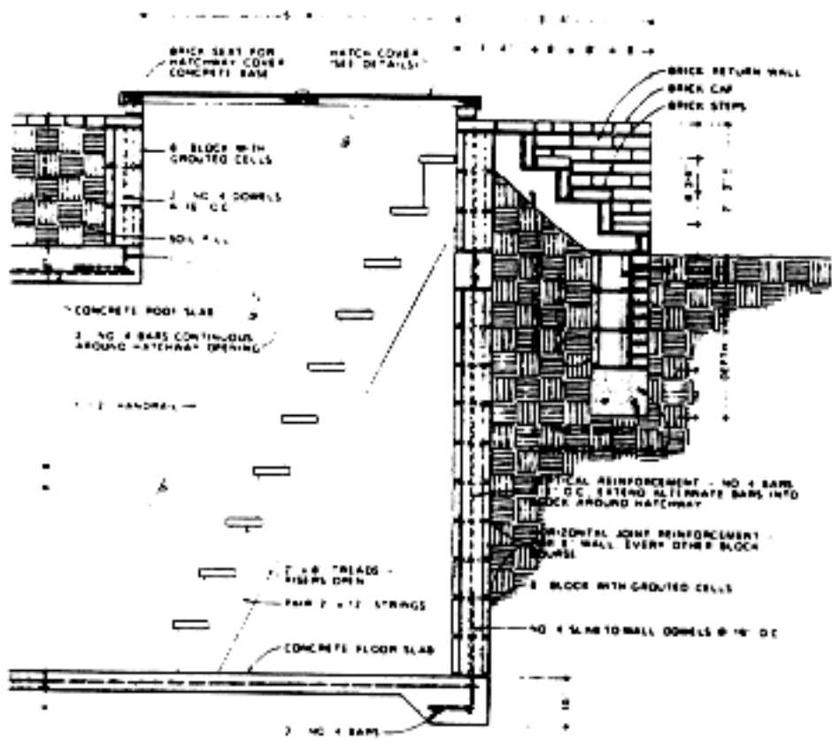
Figure 10. Section D-D at hatchway
