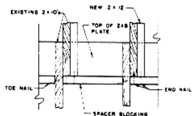
Plan detail of spacer blocking
