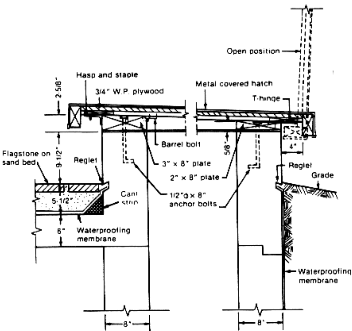
Hatch Detail
