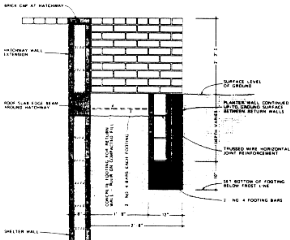
Figure 65. Showing elevation of brick coursing for return wall
