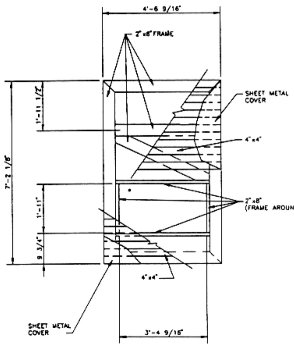
Main Hatch Cover Detail D
