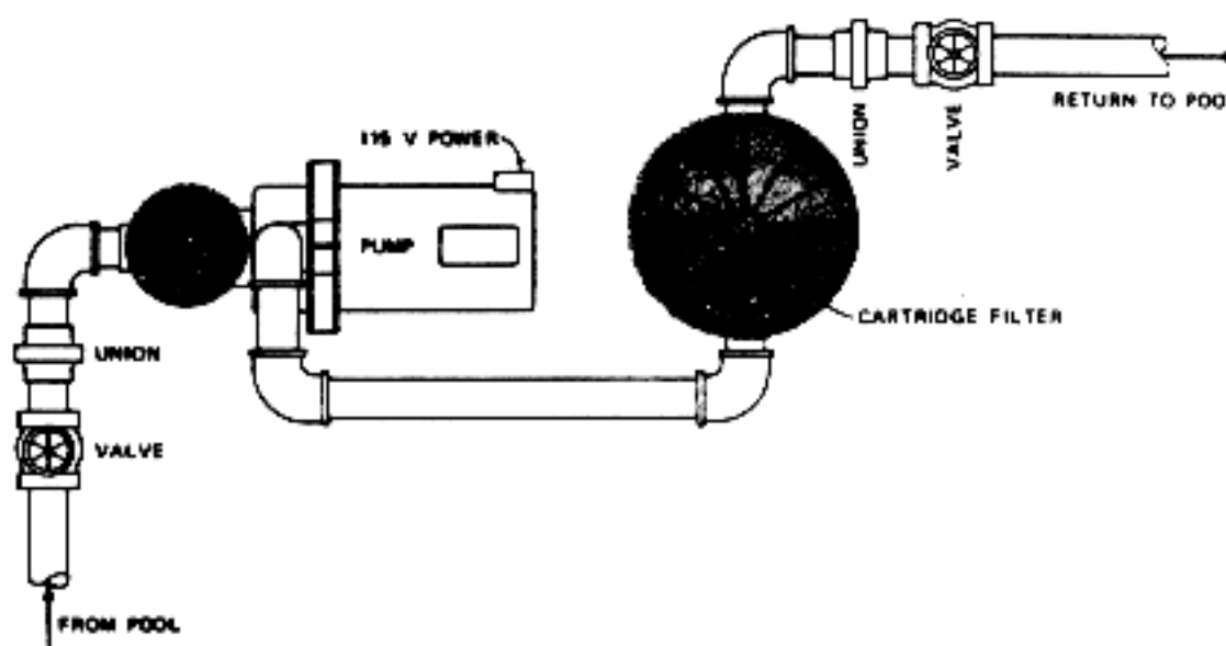
Figure 72. Schematic diagram of swimming pool filtration system
