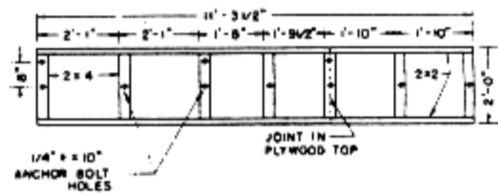
Plan of counter top frame
