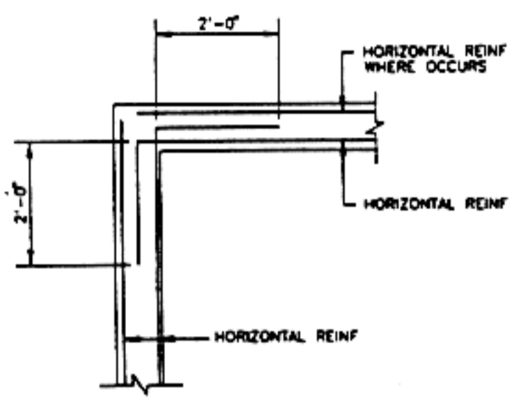
Typical wall reinf at corners
