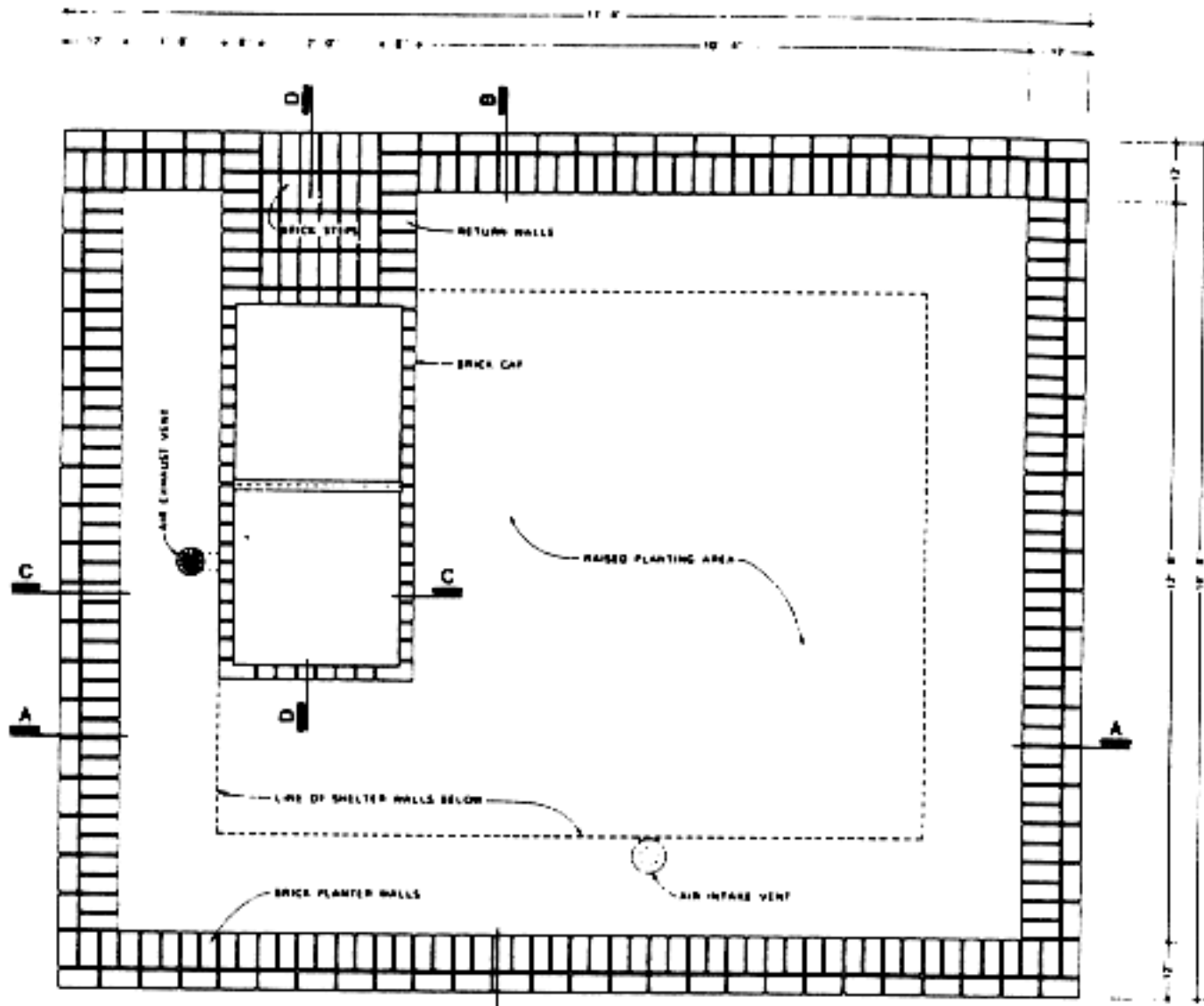
Figure 9. Dimensioned plan of the planting area at yard level
