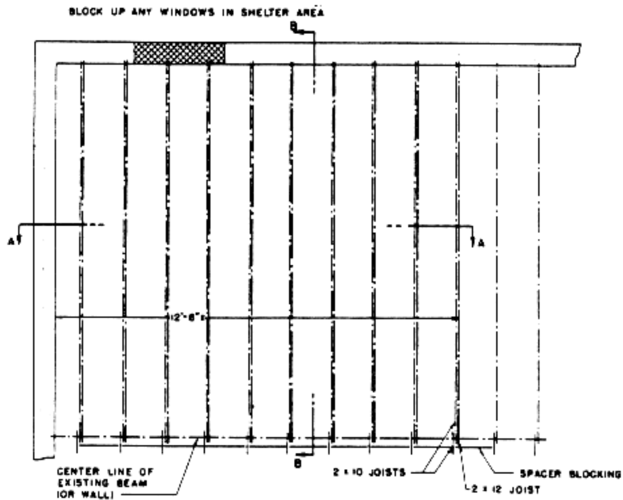
Plan for 12 X 12 Shelter
