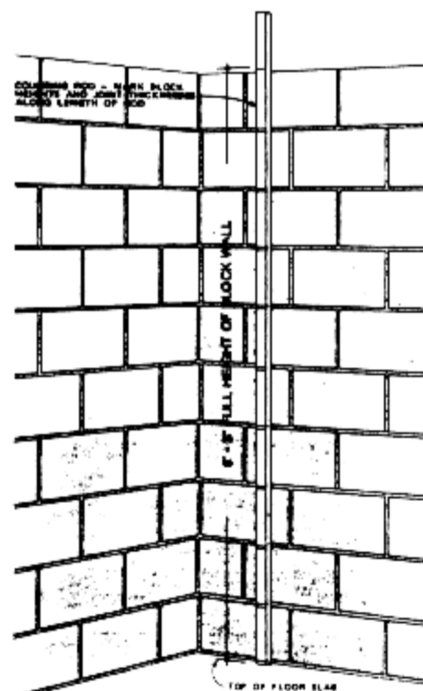
Figure 38. Preparation of a coursing rod
