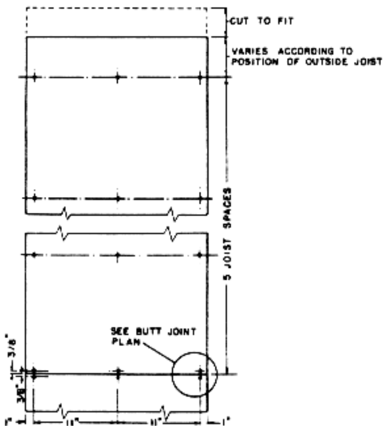
Plan of typical plywood ceiling panel
