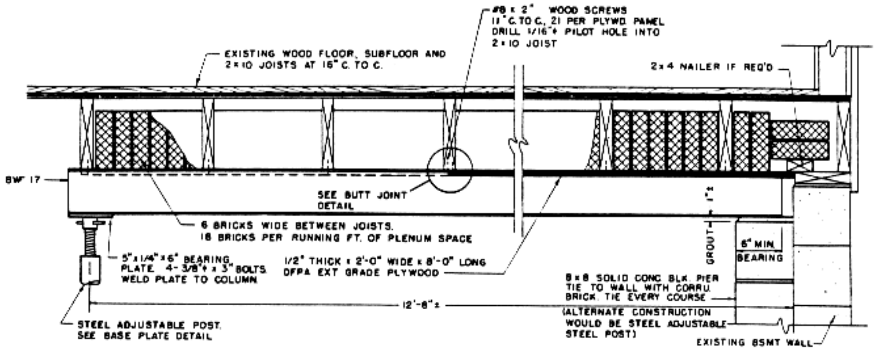
Section A
