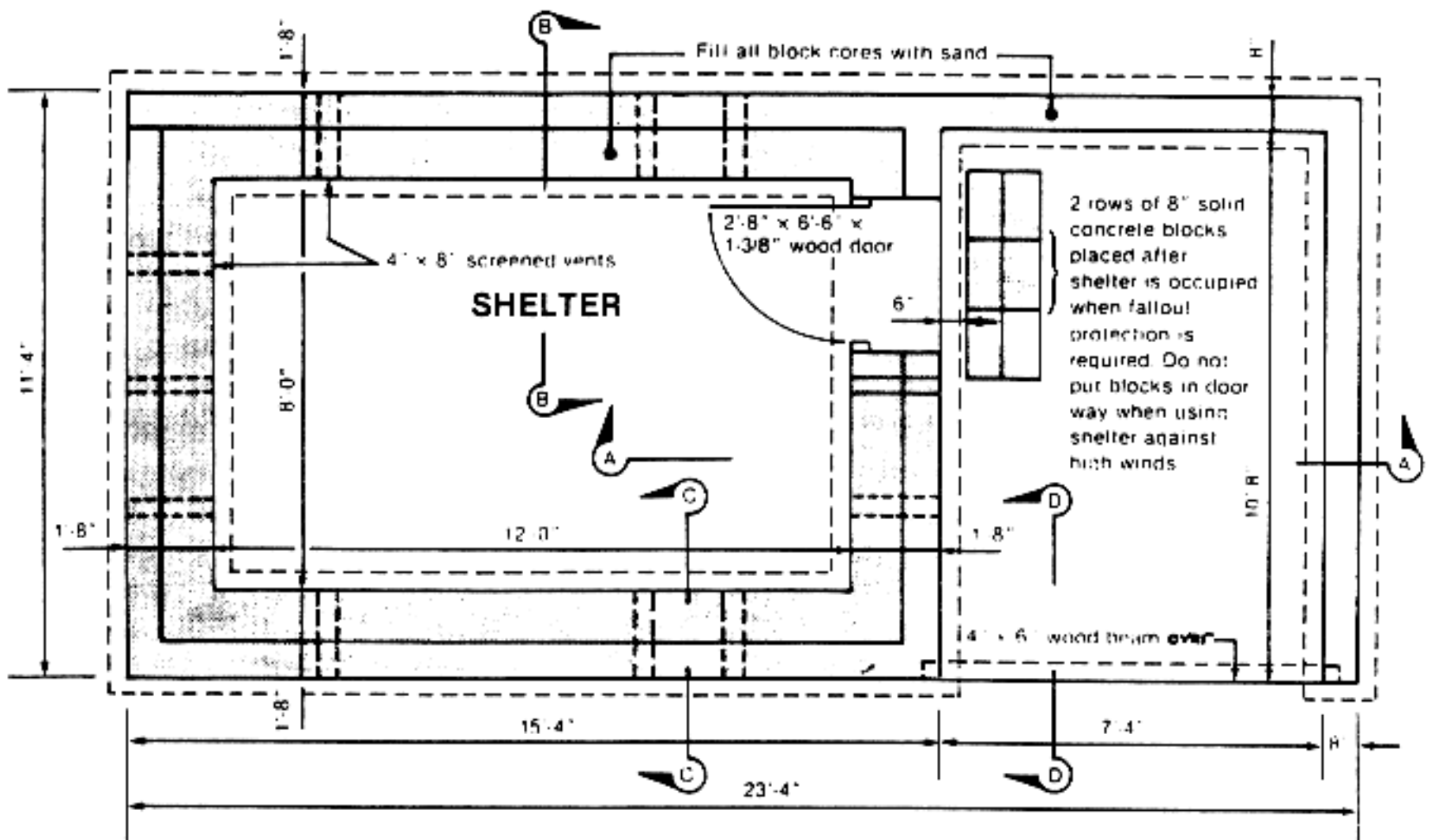
PLAN
