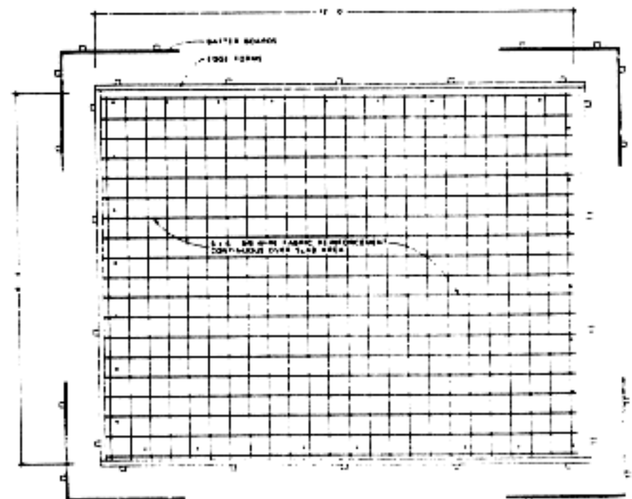
Figure 35. Placement of wire fabric reinforcement in the floor slab
