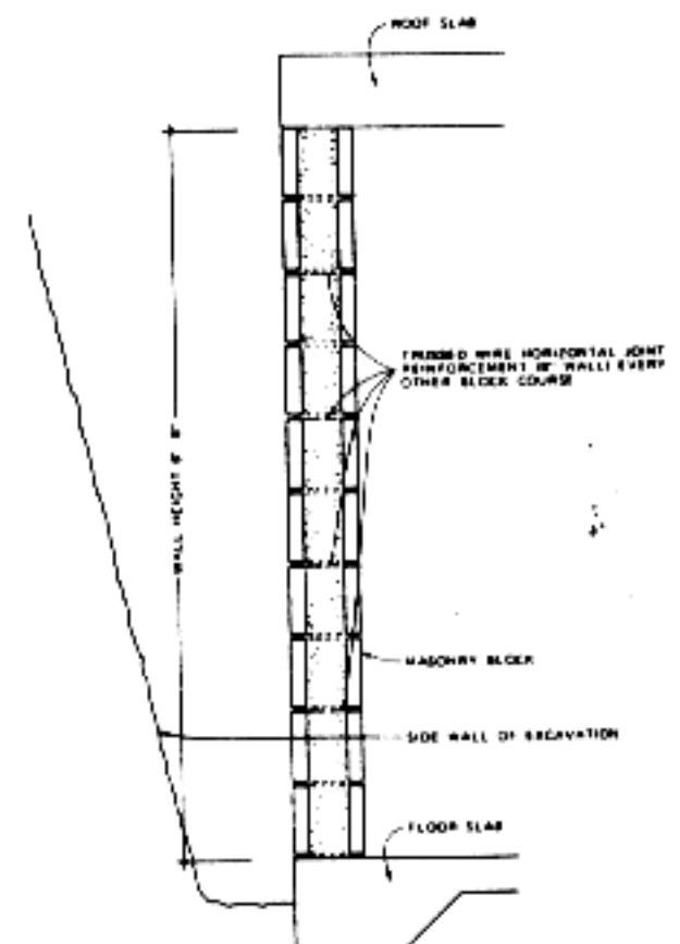
Figure 41. Shows location of horizontal joint reinforcement
