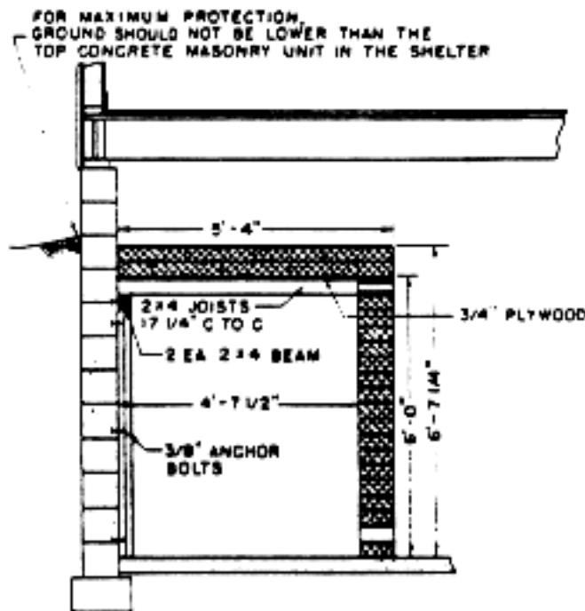
Section C
