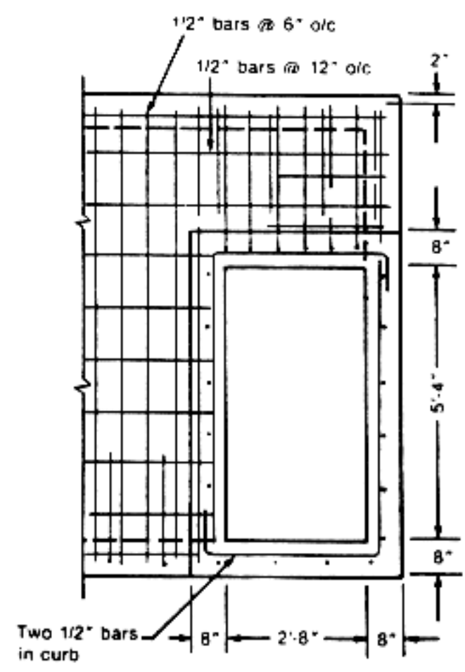
Hatch Framing
