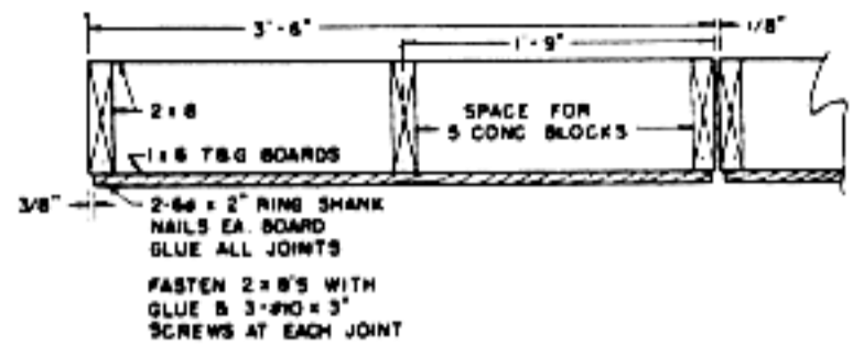
Wood case detail
