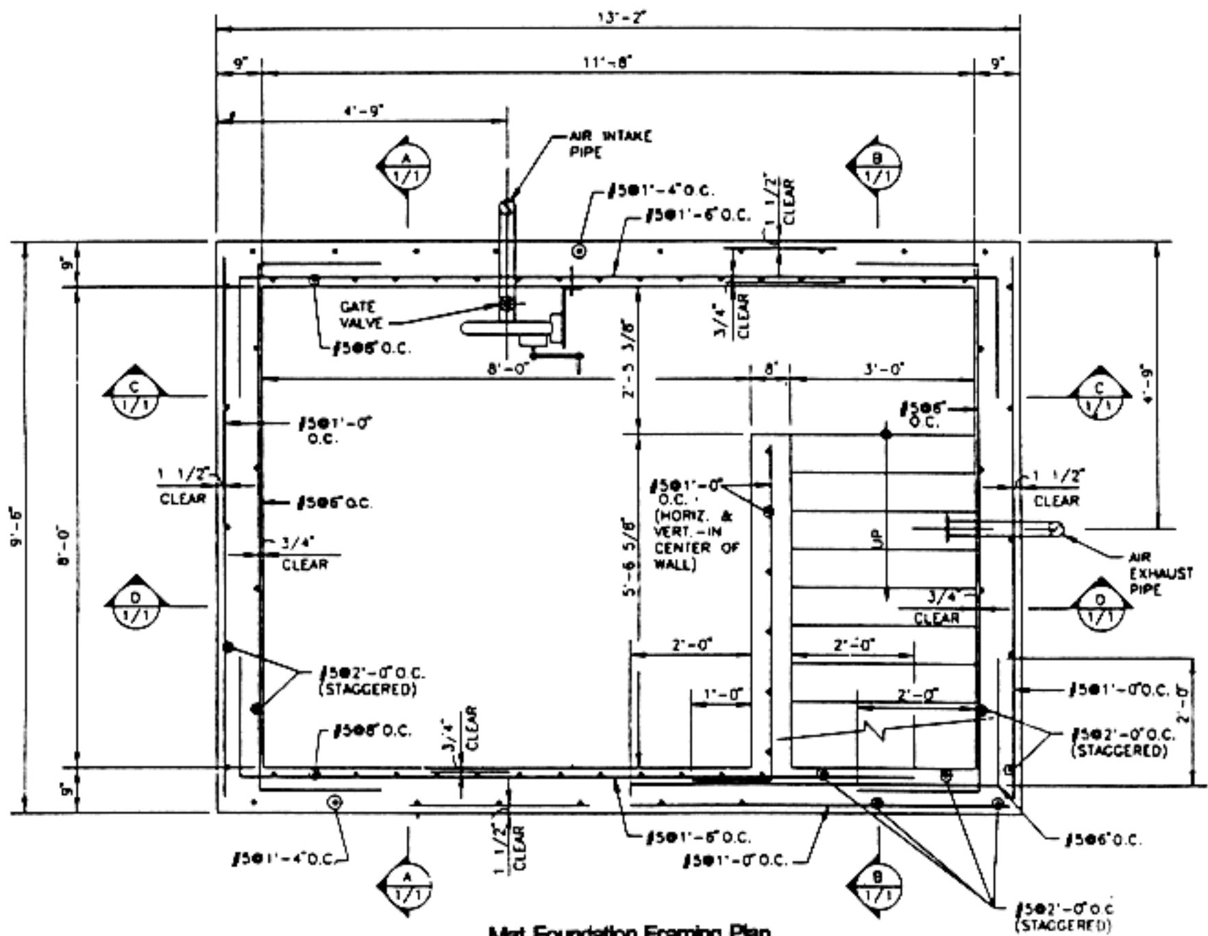
Mat Foundation Framing Plan
