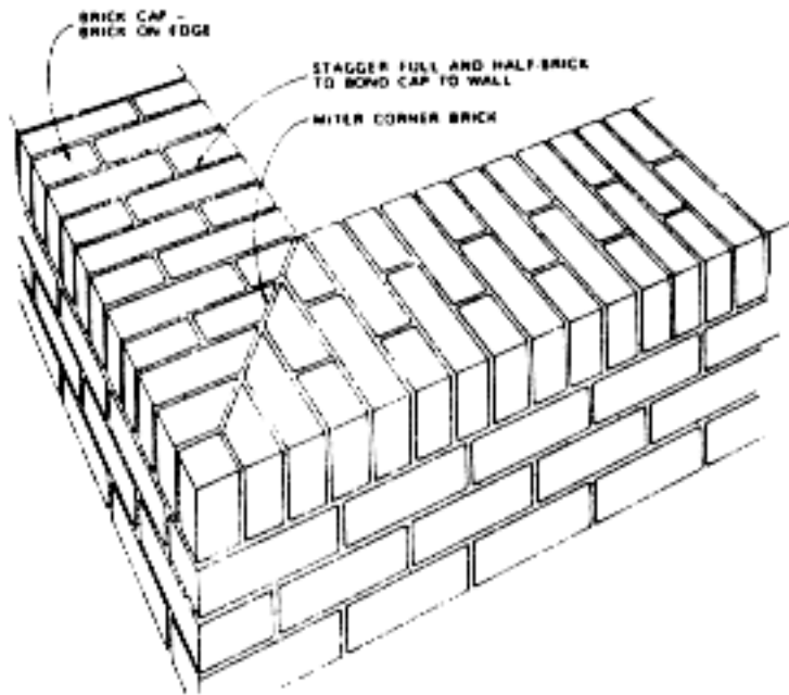
Figure 64. Alternative for brick cap of planter wall
