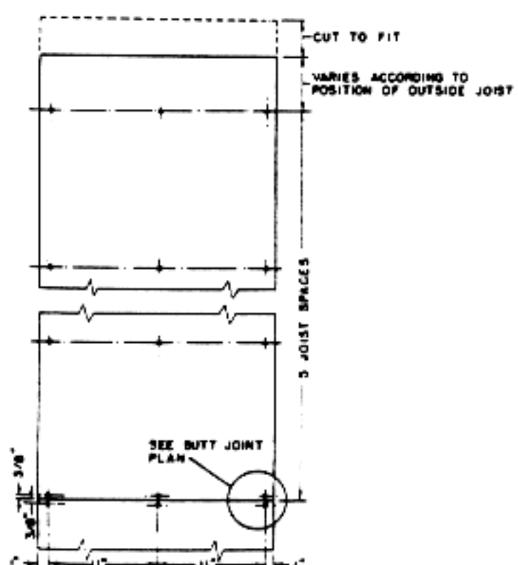
Plan of typical plywood ceiling panel
