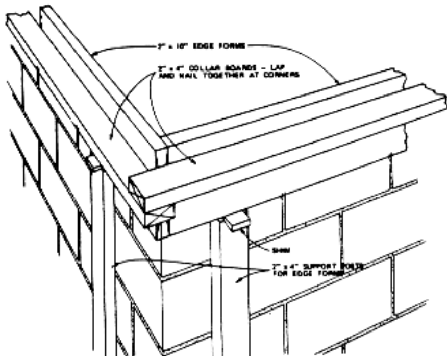
Figure 54. Retaining collar to hold forms of roof slab in place
