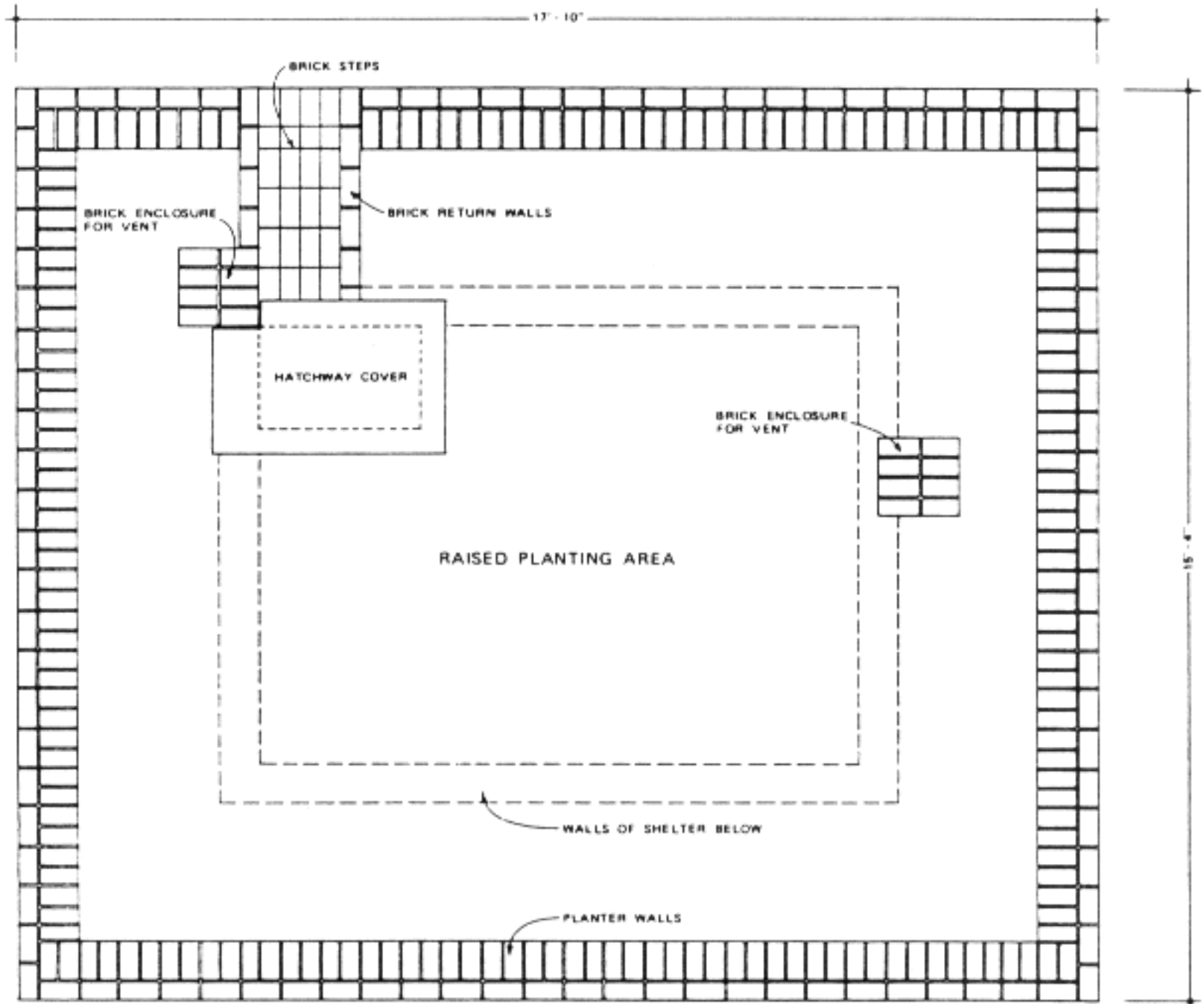
Figure 76. Yard level plan of brick planter of the swimming pool house
