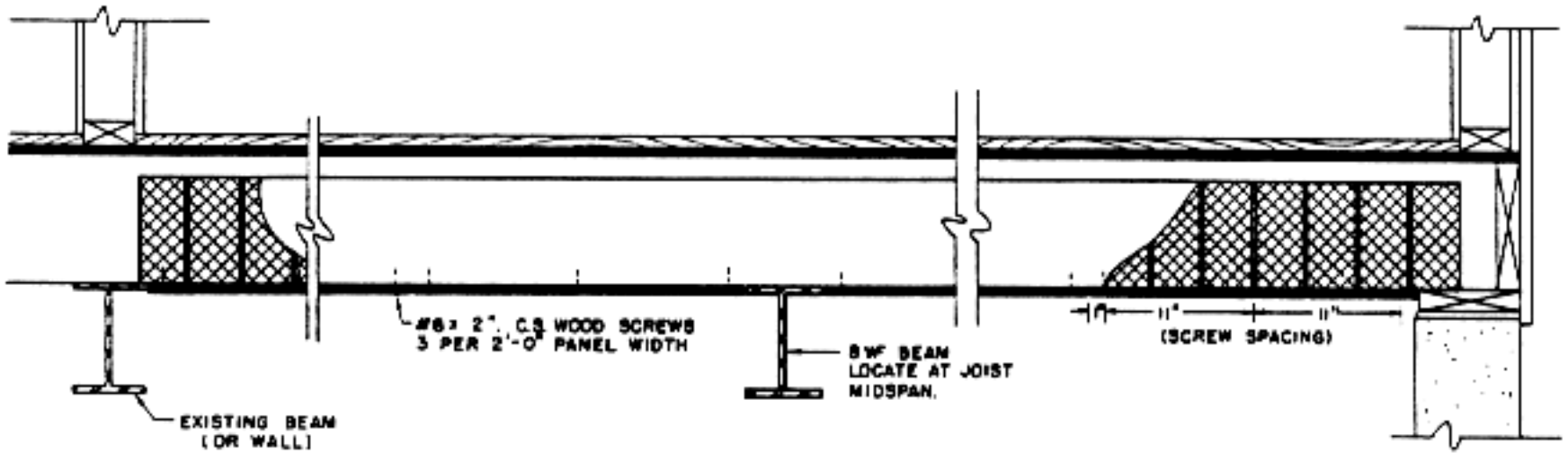
Section B
