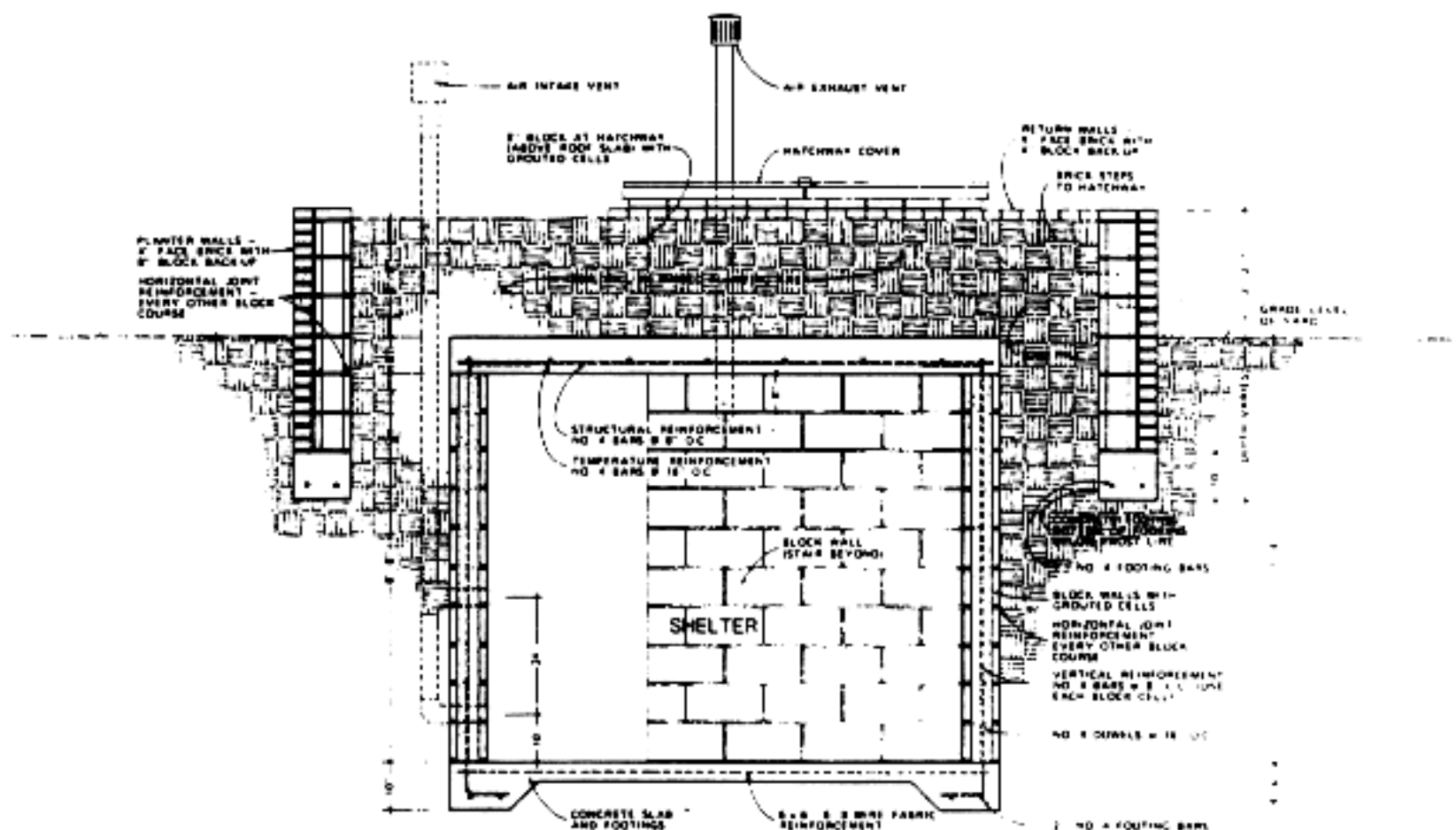
Figure 8. Dimensioned cross section B-B through the structure
