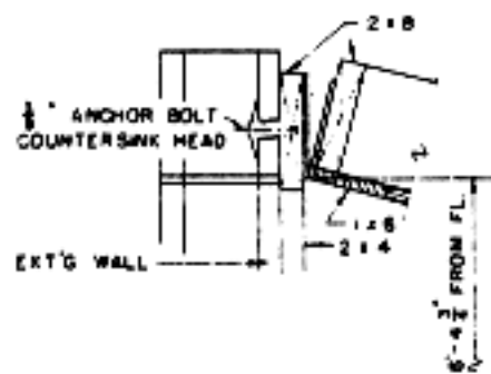
Hinge Detail
