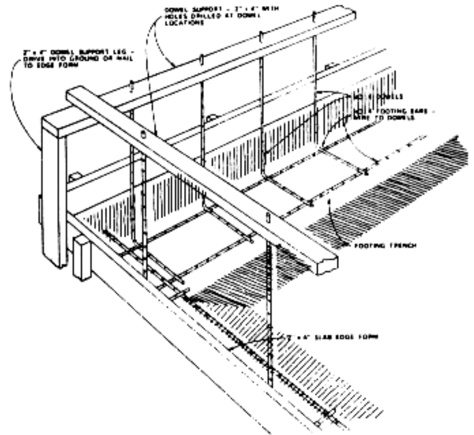
Figure 33. Placement of reinforcement steel in the slab footing
