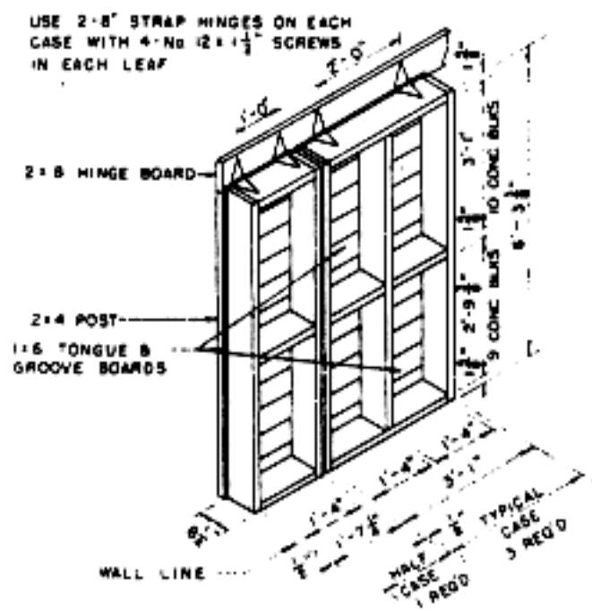
Isometric of cases
