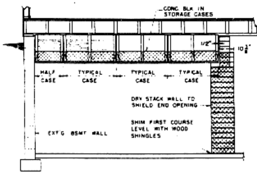
Section A-1
