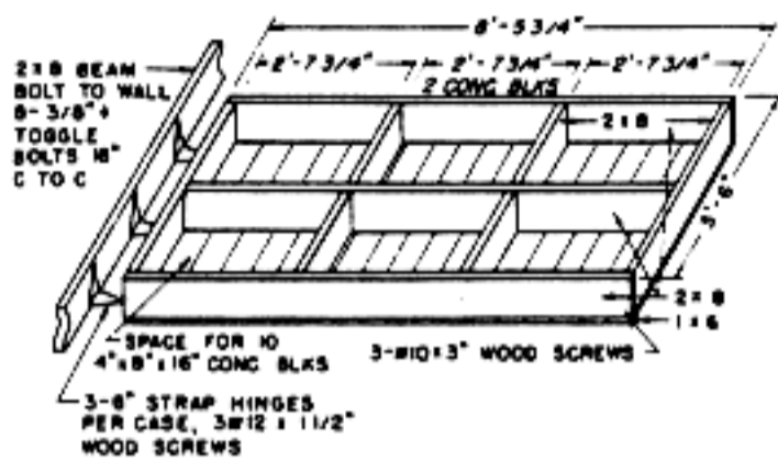
Wood case - Typical 3 cases req'd
