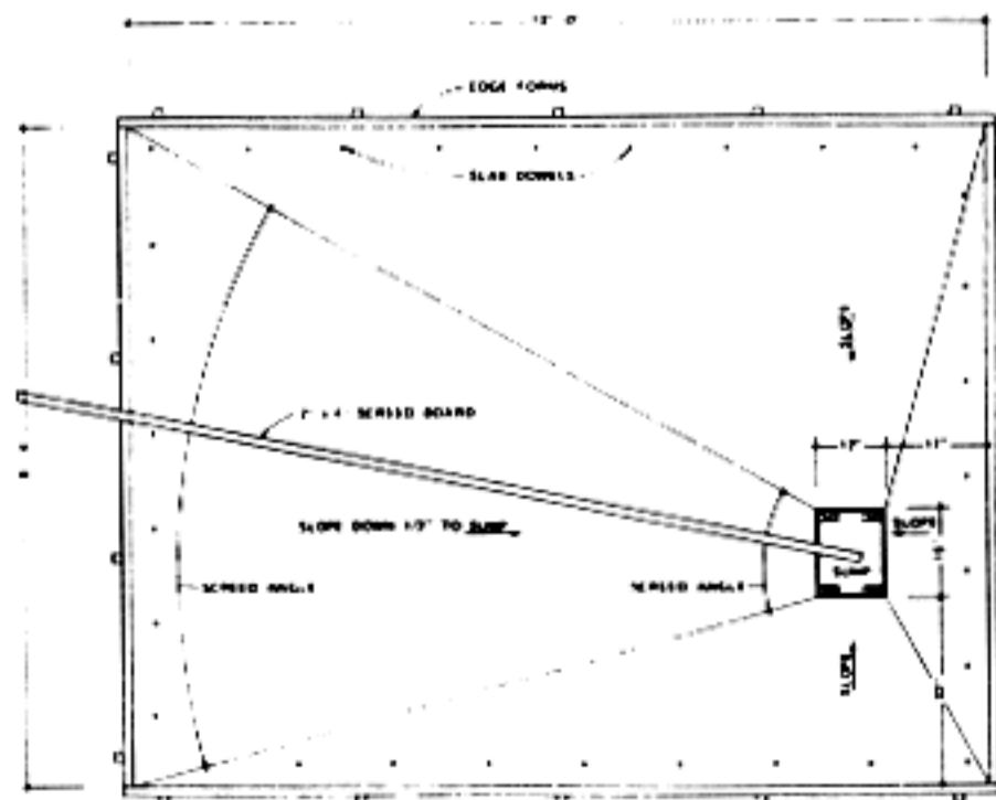
Figure 37. Screeding techniques to provide drainage slope for slabs
