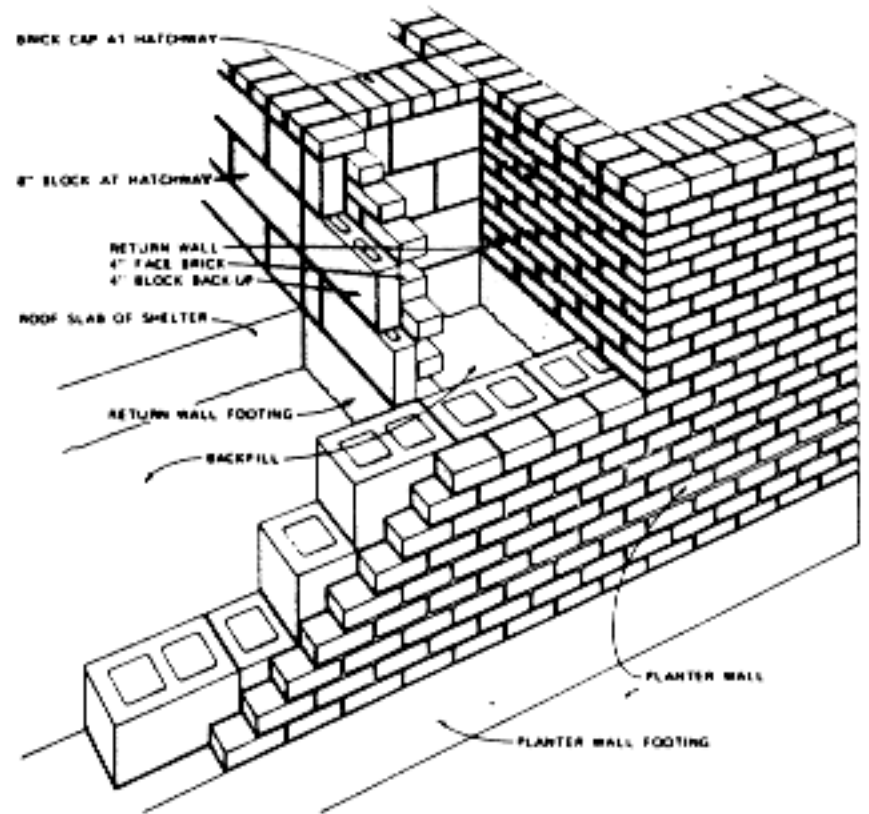
Figure 66. Diagram showing masonry work at return walls
