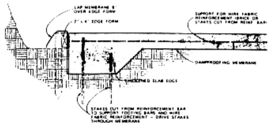
Figure 58. Placement of dampproofing membrane under floor slab
