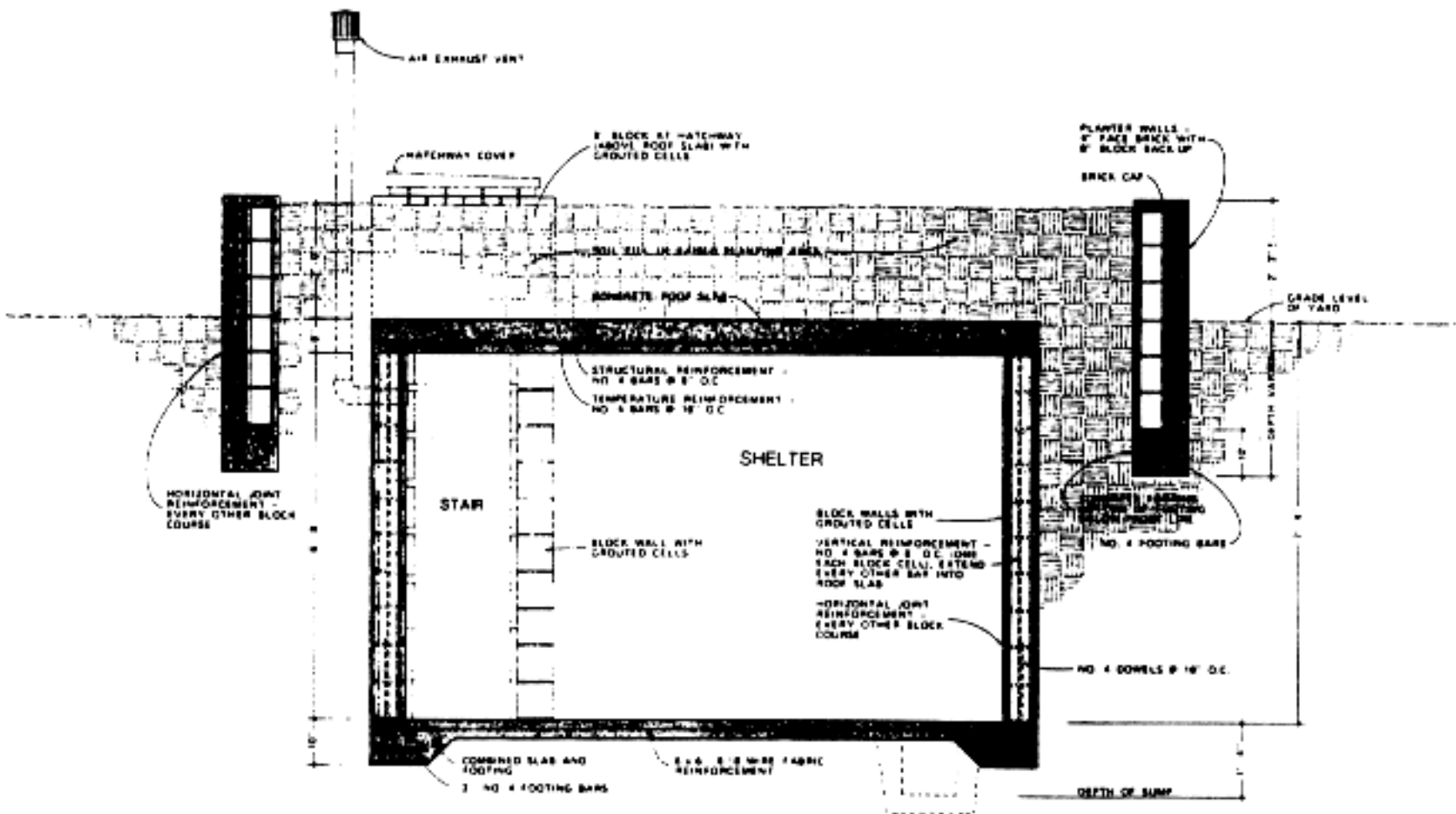
Figure 6. Dimensioned cross section A-A through the structure
