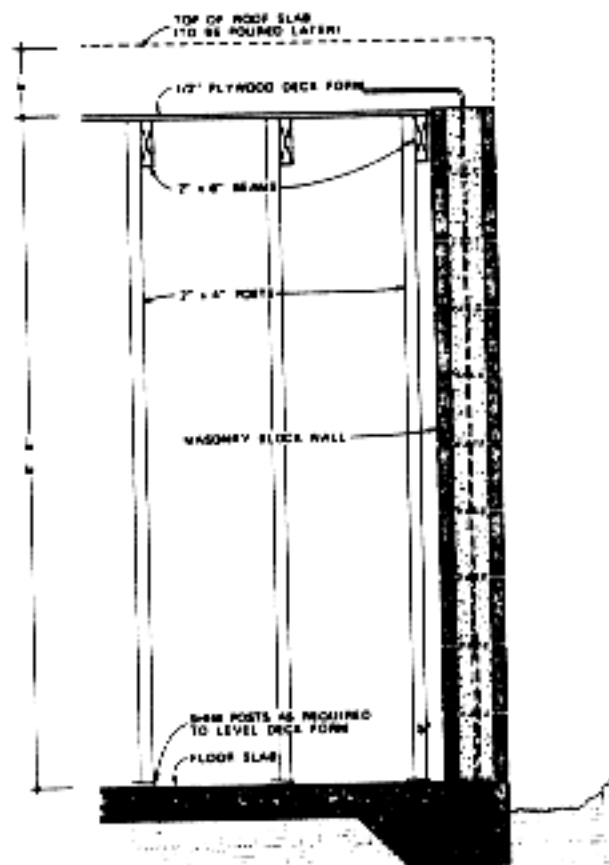
Figure 49. Cross section - placement of shoring framework
