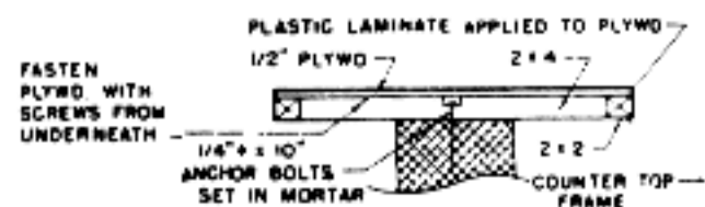
Counter top detail
