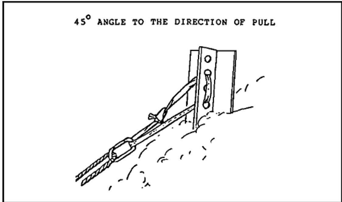
Figure 1-28. Snow Picket.
