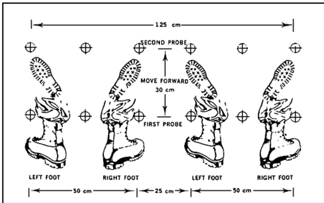
Figure 1-17. Fine Probe.
