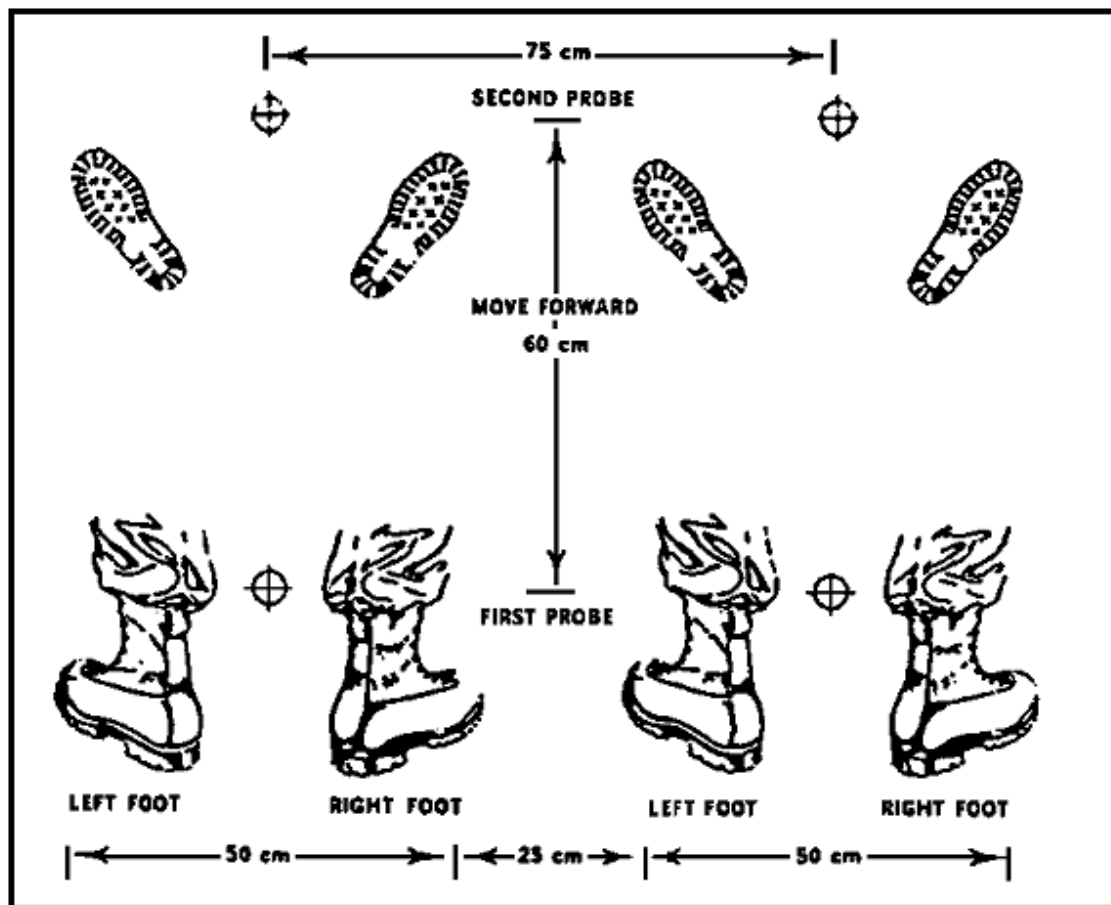
Figure 1-16. Coarse Probe.
