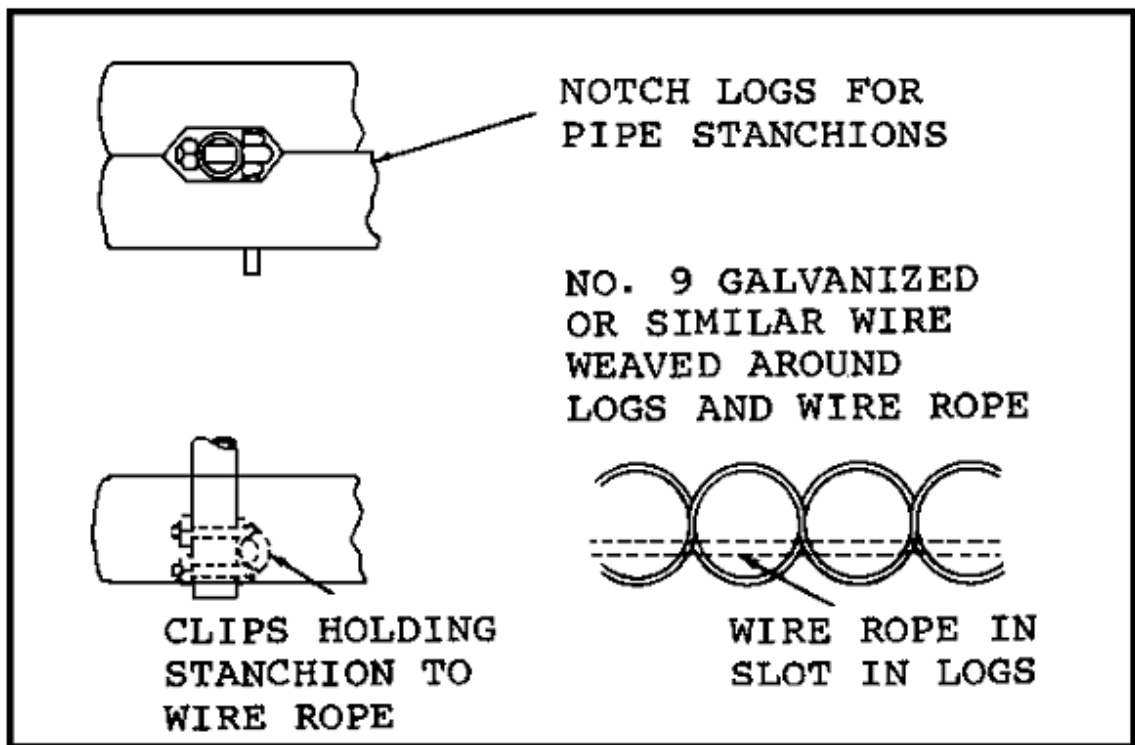
Figure 2-12. Logs Fastened in Place as a Treadway.
