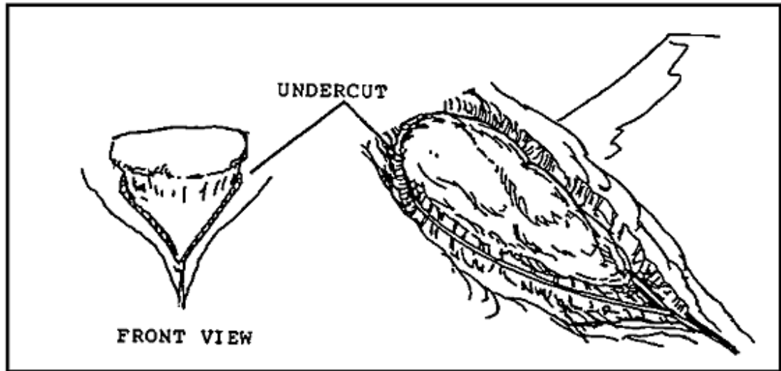
Figure 1-30. Snow Bollard.
