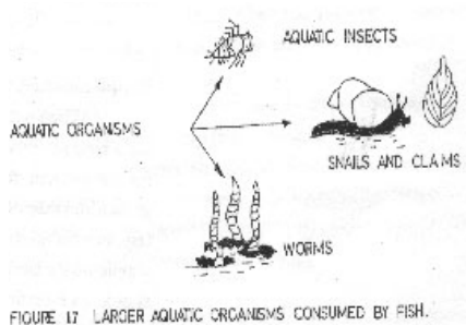
Fig 12. Lager aquatic organisms consumed by fish
