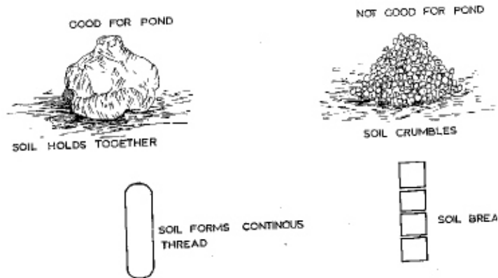
Fig 5. Testing good soil for Pond Construction
