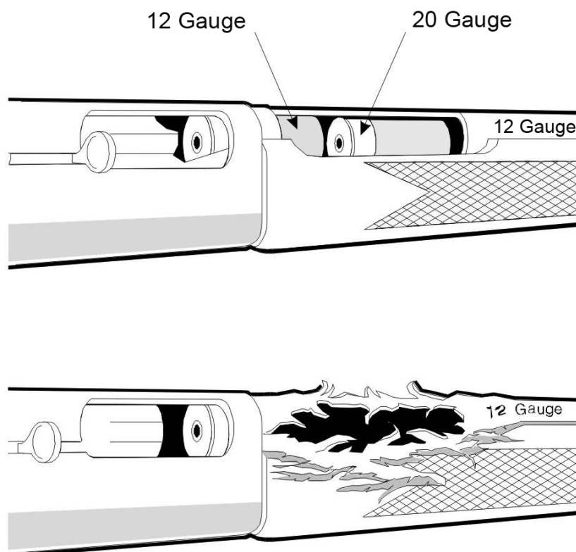
Figure 29. Exploded chamber
