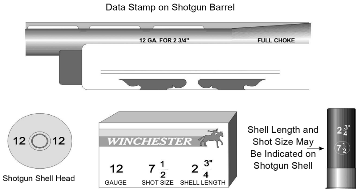
Figure 27. Shotgun shell head stamp, data stamp and ammunition box label
